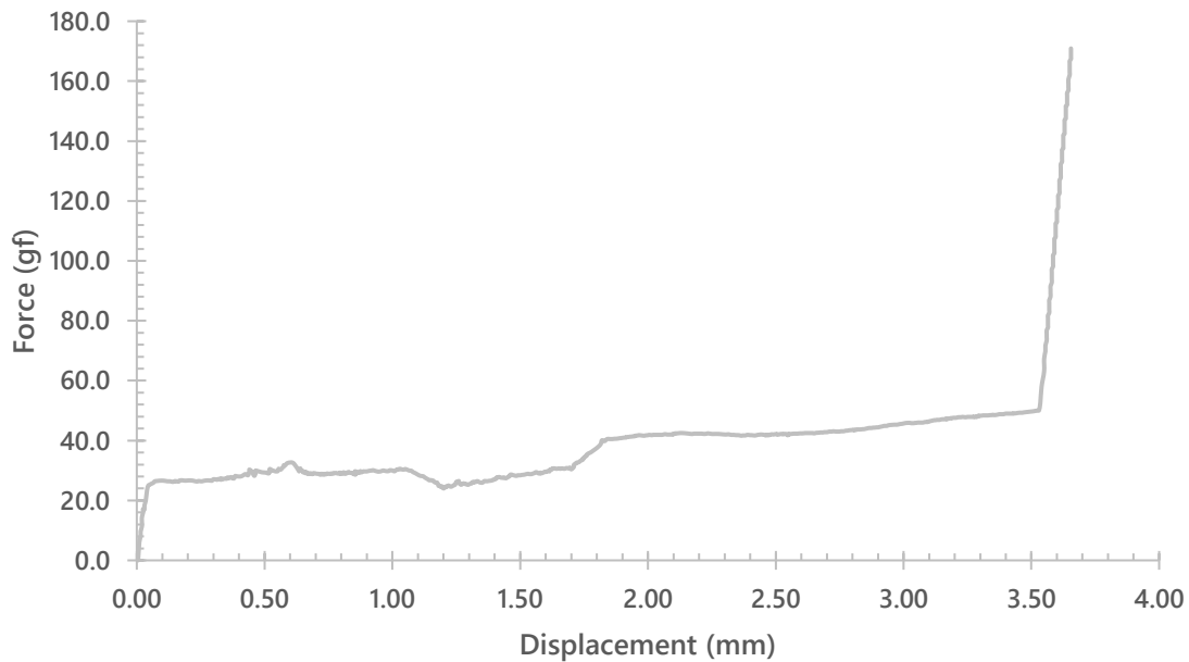
Kailh Mix-7 (Clicky Mode) (Upstroke)
